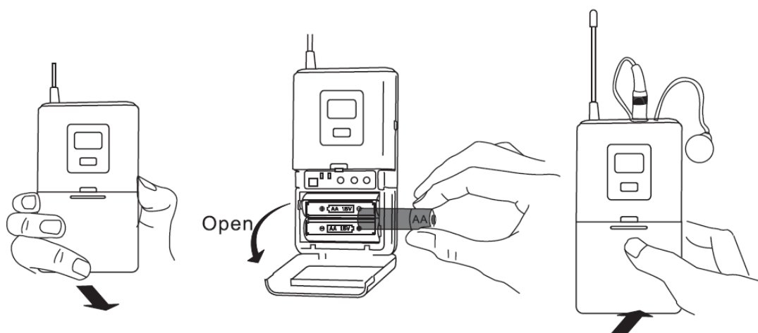
2. Make sure that you insert the battery at the right electric poles, as shown in picture.
